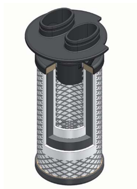
Cross section of the depth filter A
